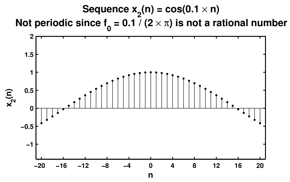
Figure 2.22: Problem P2.5.3 sequence plots
